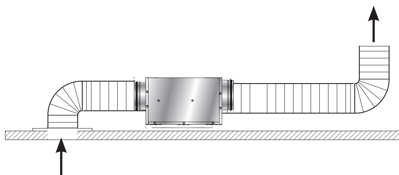
Exhaust system for ceiling
